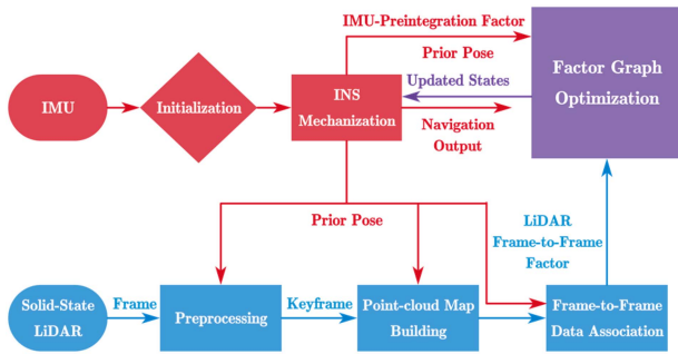
Fig. 3. System overview of the proposed FF-LINS.
