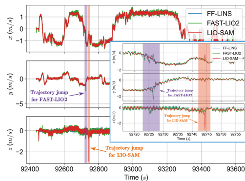
Fig. 8. Velocity curves on the R3LIVE-hkust_campus_01 dataset. The velocities are obtained from the position changes.
