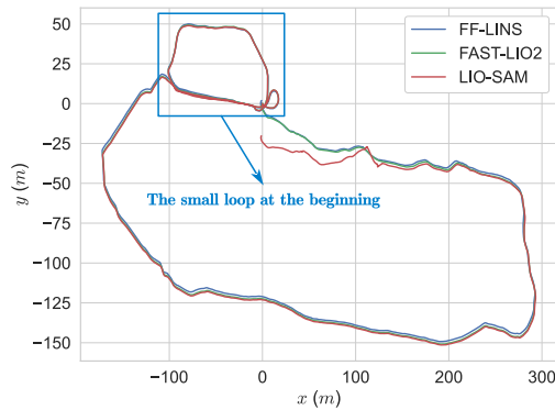
Fig. 7. Trajectories on the R3LIVE-hkust_campus_01 dataset.
