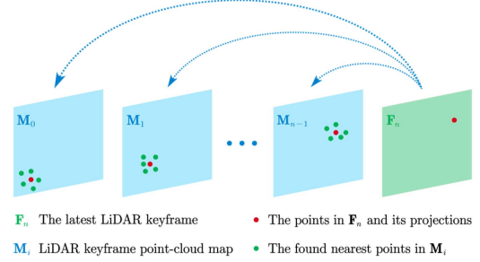
Fig. 5. Illustration of the frame-to-frame data association.
