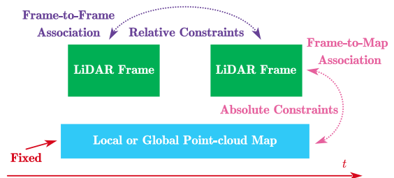
Fig. 1. Illustration of the frame-to-frame and the frame-to-map association in LiDAR navigation.
